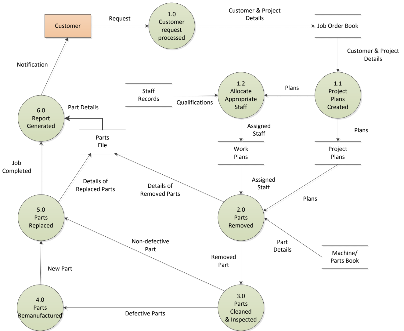
Level 1 DFD for Repair Request System
